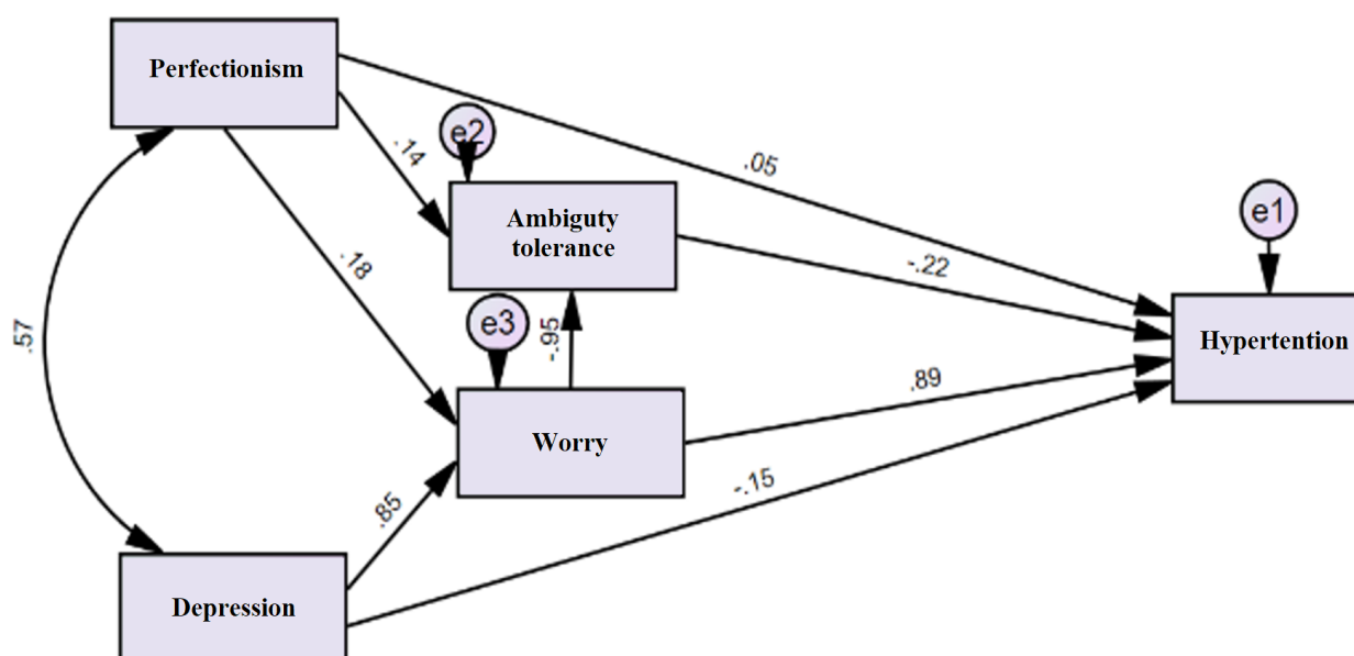
Figure 1. Path analysis model with standard coefficients for depression, perfectionism, hypertension, worry, ambiguity tolerance and problem-solving
